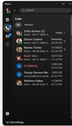
Call history
