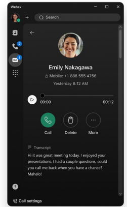
Voicemail
