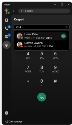
Softphone dialer
