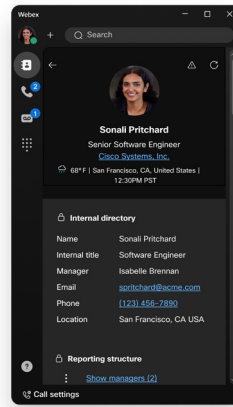
Contacts
